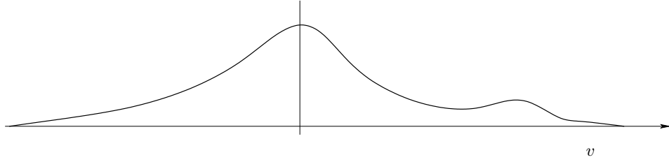
FIGURE 3.5. Bump-on-tail instability: For a given length of the box, there will be linear instability for some large enough secondary bump. Conversely, if a non-monotone velocity distribution is given, there will be instability for some large enough size of the box.
