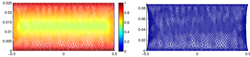
FIG. 8.3. Uniaxial tension of a thin bar, \Omega = (-0.5, 0.5) \times (0, 0.025) , \lambda = 3.5 , p = 3 .
