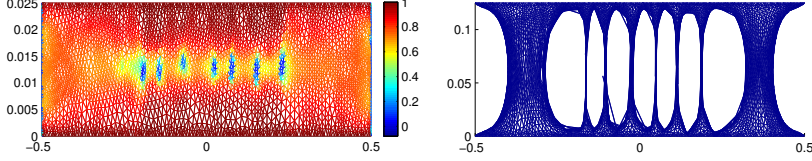
FIG. 6.4. An even thinner bar: (-0.5, 0.5) \times (0, 0.025) , \lambda = 5 .
