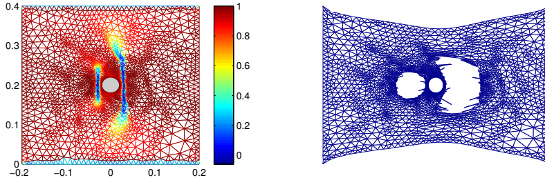
FIG. 7.3. A square with a rigid inclusion, \lambda = 1.485 .
