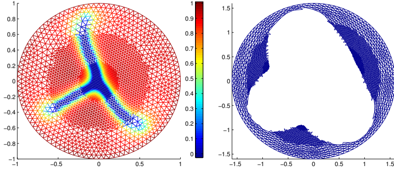
FIG. 8.2. Fracture of a perfect ball, \lambda = 1.6 , \varepsilon = 0.025 , p = 3 .
