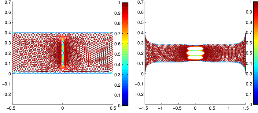
FIG. 4.6. A slab with three micro-holes, \lambda = 3 .
