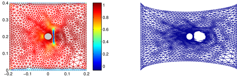
FIG. 7.2. A square with a rigid inclusion, \lambda = 1.48 .
