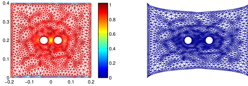
FIG. 7.5. A square with two rigid inclusions, \lambda = 1.4 .
