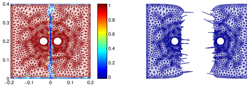
FIG. 7.6. A square with two rigid inclusions, \lambda = 1.41 .
