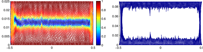
FIG. 8.4. Uniaxial tension of a thin bar , \Omega = (-0.5, 0.5) \times (0, 0.025) , \lambda = 3.6 , p = 3 .
