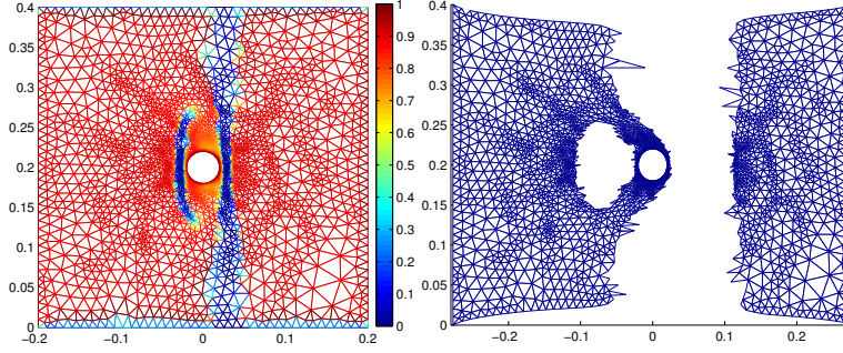
FIG. 8.5. Uniaxial tension of a square with a rigid inclusion , \lambda = 1.385 , \varepsilon = 0.001 , p = 3 .
