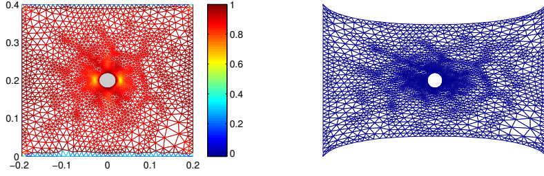
FIG. 7.1. A square with a rigid inclusion, \lambda = 1.475 .
