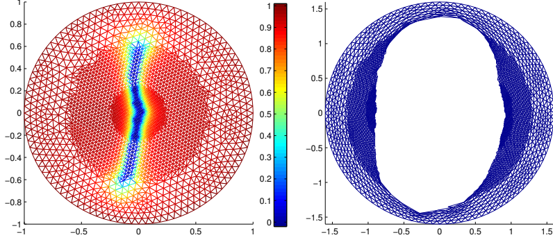
FIG. 8.1. Fracture of a perfect ball, \lambda = 1.6 , \varepsilon = 0.025 , p = 2 .
