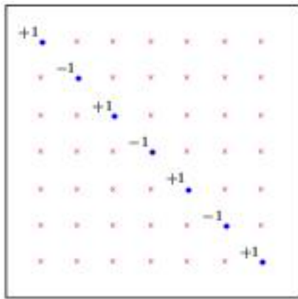
Figure 1: The eigenvector for the 5-point finite difference scheme for the laplacian in the square, with eigenvalue \lambda = 4/h^2 , taking alternating values \pm 1 along a diagonal and vanishing everywhere else in the domain.
