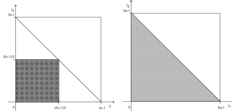
FIGURE 6. On the left, the black area represents the frequencies involved in J_h(1/2) ; On the right the dashed area represents the the frequencies involved in I_h(2) .
