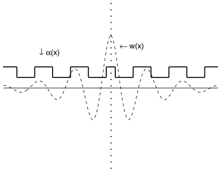
Fig. 1. Construction of \alpha and w satisfying (2.11).
